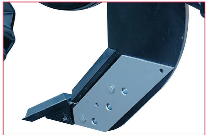
1 3/4"-wide triangular-shaped wearbars extend shank life and minimize pulling resistance. Optional side-mounted shank protectors enhance shank life and performance.
