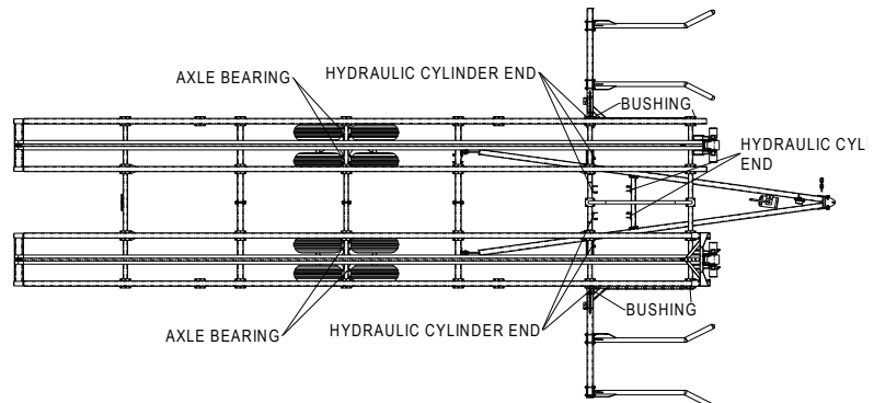
LUBRICATION ILLUSTRATION
