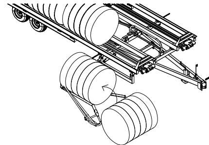
BALE DEFLECTOR
