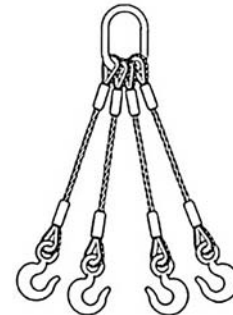
VERTICAL CHOKER BASKET
